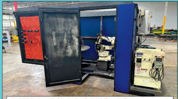
(2) OTC Rotary Table Robotic Welding Cells
